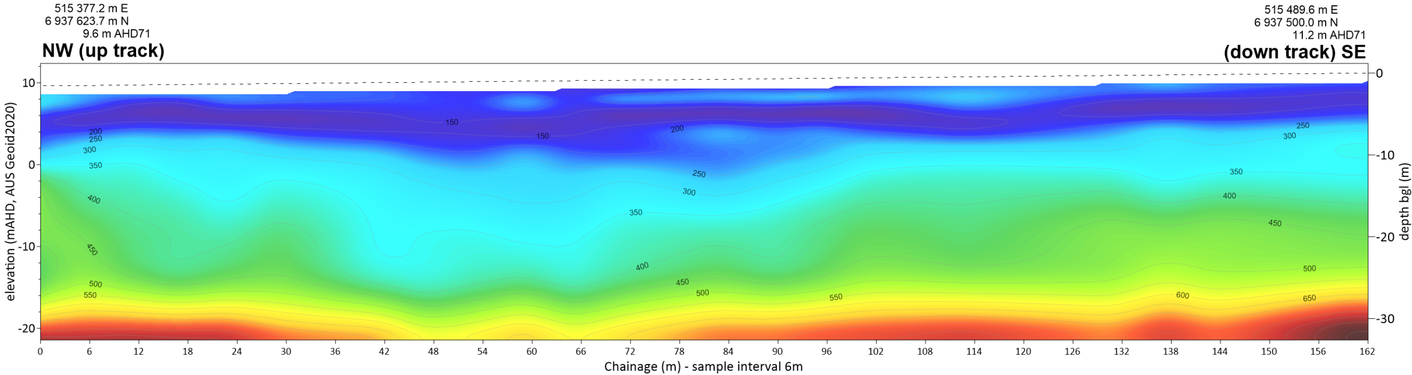
Seismic Line MASW AU-GP 163-1
